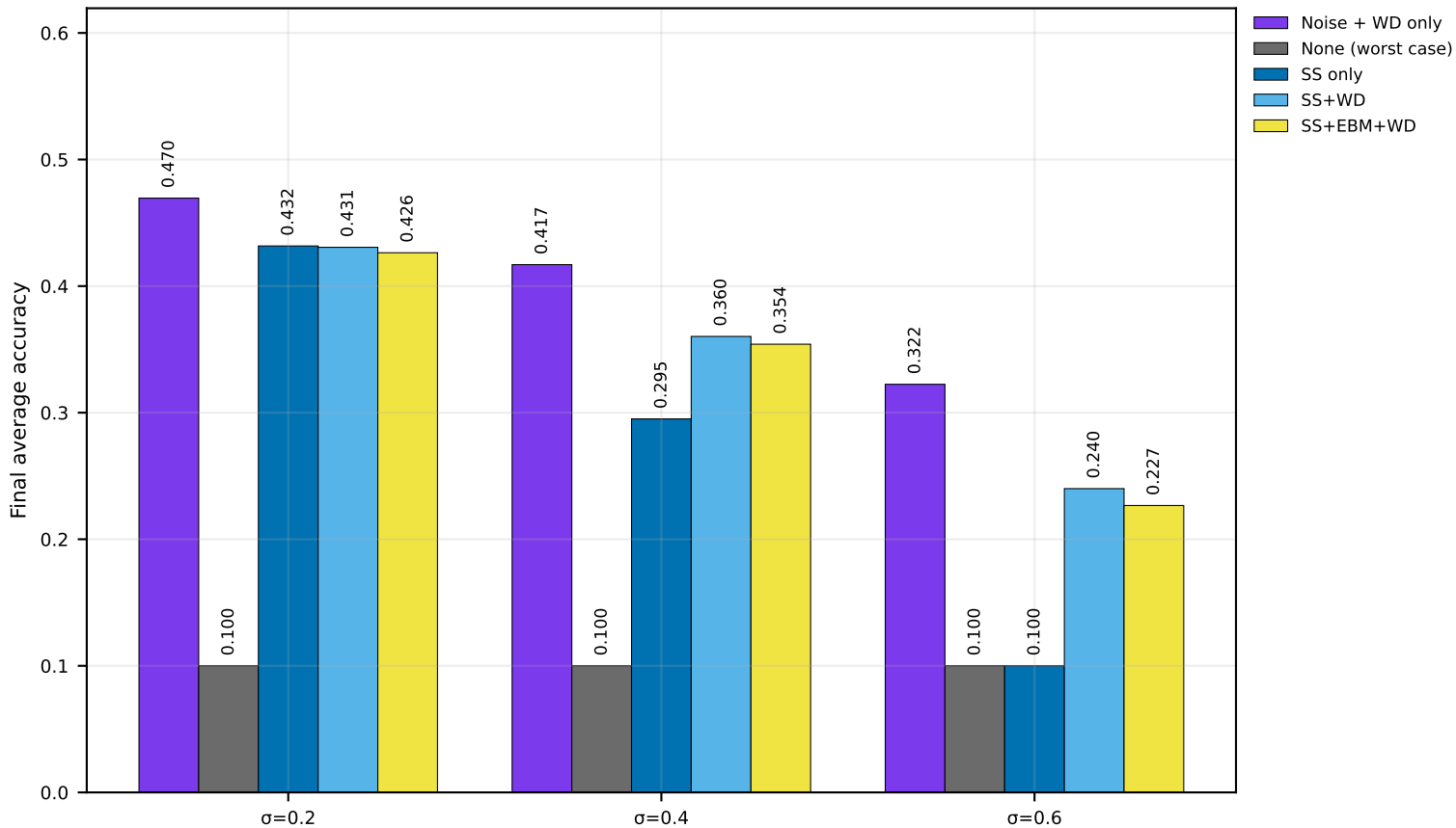
Ablation Groups | CIFAR-10 | CART | seed=avg of 4 seeds (nonIID)
